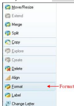
Figure 4-17: Choose format
